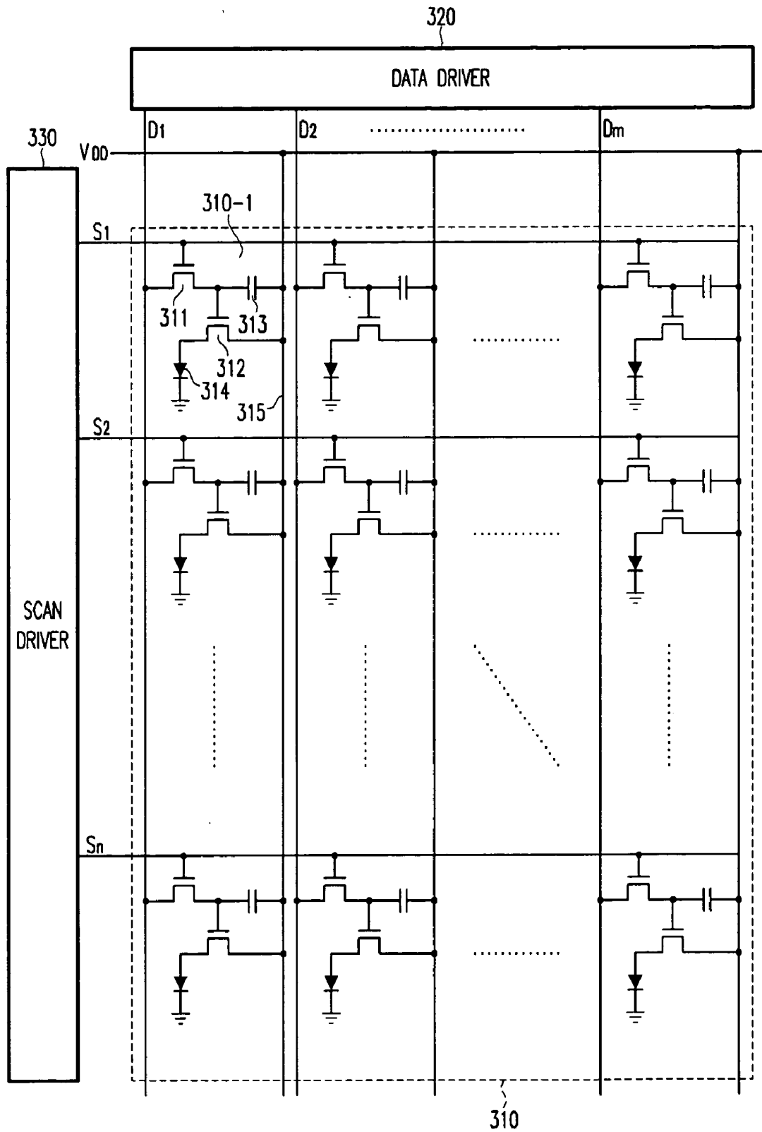
FIG. 3 Prior Art
